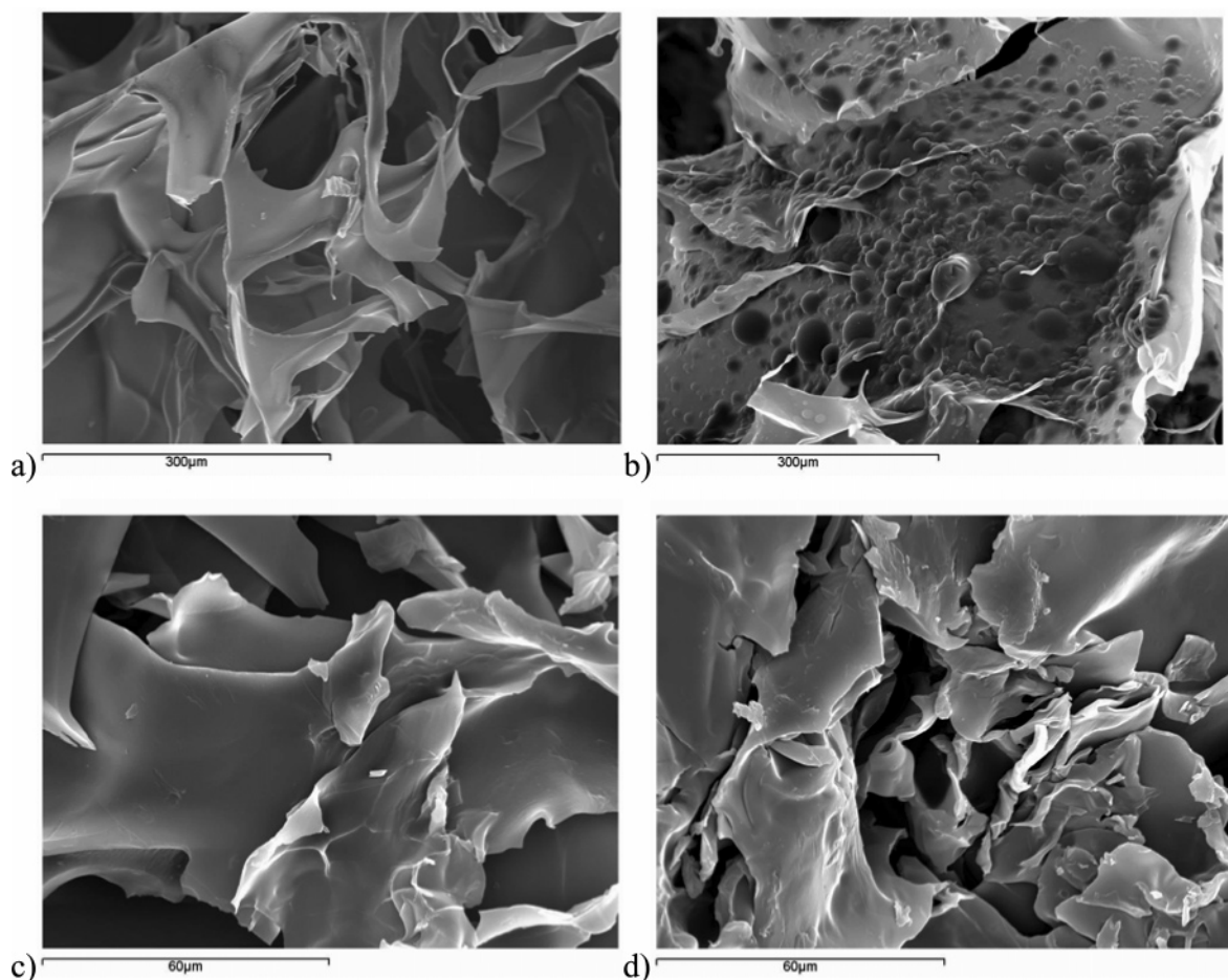
Figure 7. Scanning electron micrographs of dry CS-GNP hydrogels at R = 0.25 : (a) control CS-GNP hydrogel; (b) CS-GNP- o -xylene complex before extraction; (c and d) corresponding micrographs for the same materials as in parts a and b, respectively, after acidic aqueous extraction. (Magnification is as given in the scale bars.)
