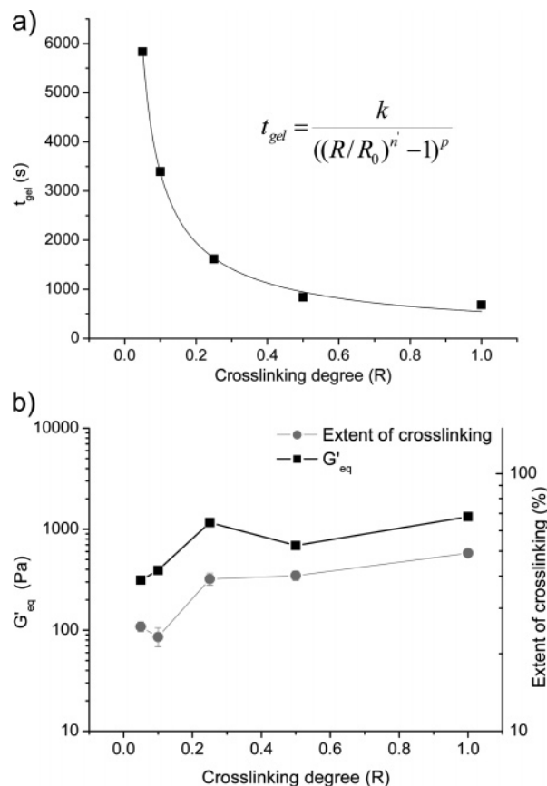
Figure 3. (a) Variation of t_{\text{gel}} ( \omega = 1 \text{ rad s}^{-1} , \gamma = 10\% , T = 40^\circ \text{C} ) with R for CS–GNP gels at a constant chitosan concentration (1.5% (w/w) in 0.1 M acetic acid) and the nonlinear best fit of Ross-Murphy's model, (b) Dependence of G'_{\text{eq}} at 1.8t_{\text{gel}} ( \omega = 1 \text{ rad s}^{-1} , \gamma = 10\% , T = 40^\circ \text{C} ) and extent of cross-linking on R for gels as in part a.
