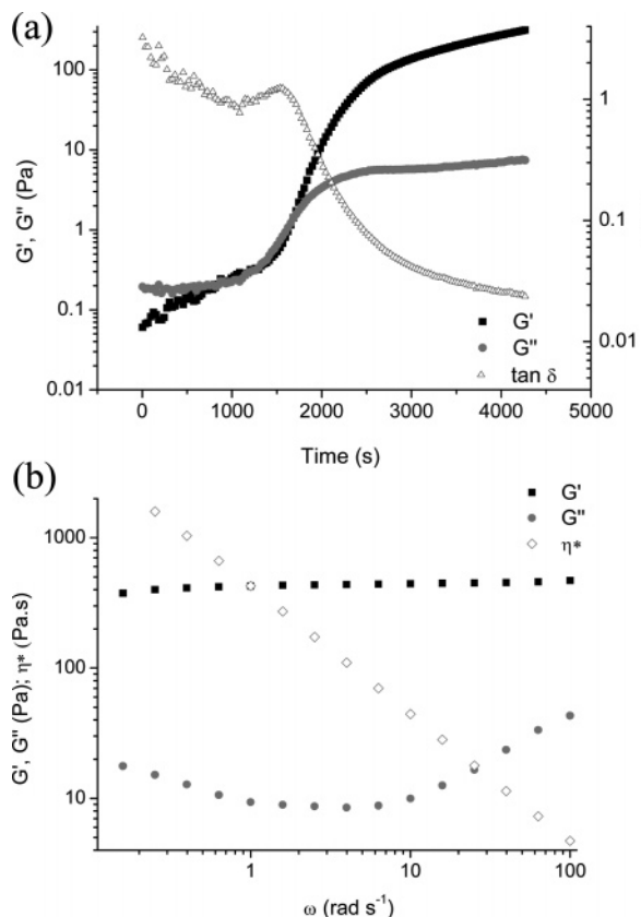
Figure 2. (a) Variation of the viscoelastic moduli, G' and G'' ( \omega = 1.0 \text{ rad s}^{-1} , \gamma = 10\% ), of a CS–GNP hydrogel formed from a chitosan solution (1.5% (w/w) in 0.1 M acetic acid, R = 0.5 , T = 40^\circ \text{C} ). (b) Frequency dependence of G' , G'' , and the complex viscosity, \eta^* ( \gamma = 10\% ), of the gel in part a after 1.5 h.
