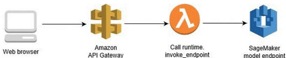
Figure 4.6: AWS architecture of Sagemaker with lambda.
