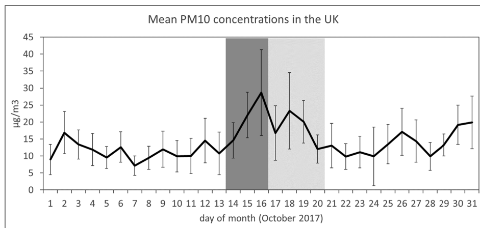
Fig. 4. Mean daily PM 10 concentrations with respective standard deviations in October 2017 from 65 air quality monitoring stations in the United Kingdom (England, Wales, Scotland and Northern Ireland). Gray bars correspond to wildfire smoke days without dust (light gray) and to wildfire smoke days with dust (dark gray).
