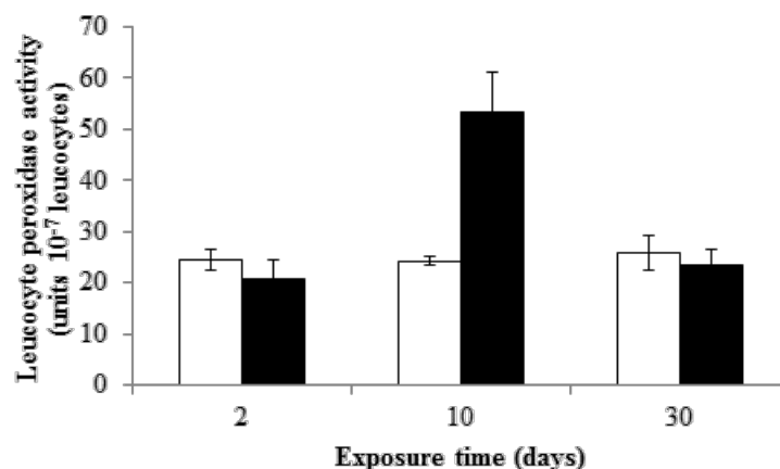
Fig. 3. Leucocyte peroxidase activity (units 10^{-7} leucocytes) in head-kidney leucocytes of gilthead seabream specimens unexposed (control; white bars) or exposed to 5 \mu M of arsenic (black bars). Bars represent the mean \pm S.E. (n=6). Asterisk denotes significant differences between unexposed and exposed groups ( P \leq 0.05 ).
