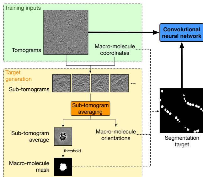
Figure 2: Target generation strategies for training. DeepFinder includes a graphical user interface (see Supplementary Fig. 6) to guide users throughout the learning procedure, from selecting the 3D coordinates of macromolecules to voxel-wise annotation. Strategy 1 (left): voxel-wise annotations are obtained from position-wise annotations using a subtomogram averaging procedure. Subtomogram averaging is a registration algorithm that produces higher resolution structures by averaging thousands of aligned subvolumes containing the molecular species. Subtomogram volumes are extracted at the annotated positions, aligned and finally averaged. The alignment procedure outputs the object orientations, while the averaging process provides a density map of the macromolecule with greatly reduced noise and missing wedge artifacts. From this density map, it is possible to create a binary mask of the macromolecule by thresholding the averaged subtomogram. The resulting mask is pasted into an empty volume at each annotated position with the estimated 3D orientation, and the resulting volume with well-delineated macromolecules is then used as a target to train the 3D CNN parameters. Strategy 2 (right): the macromolecule masks are approximated and replaced by sphere masks. Hence, the subtomogram averaging procedure is bypassed and the target generation process is much faster. However, the training targets contain more "label noise".
