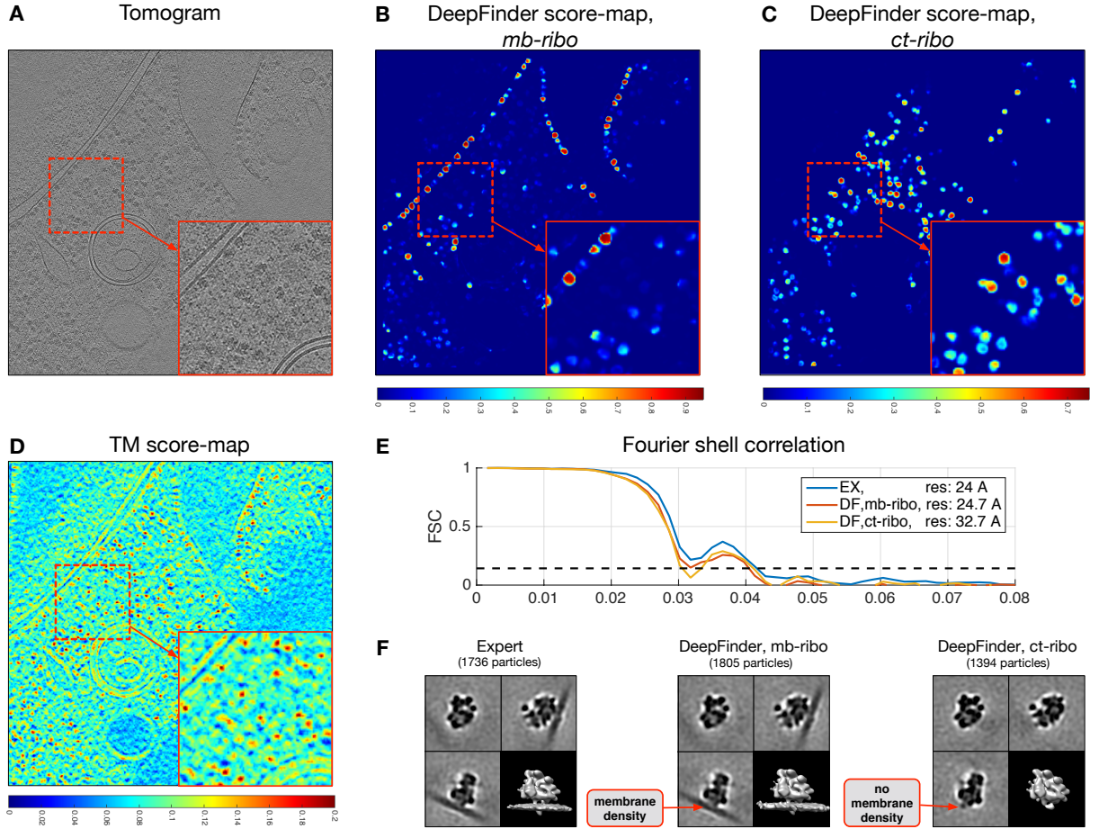
Figure 4: Comparison of score-maps obtained with template matching and DeepFinder and analysis of structural resolution through subtomogram averaging (Dataset #2). (A) Experimental cryo-electron tomogram depicting a Chlamydomonas reinhardtii cell (Dataset #2, see Methods). (B,C) Localizations of mb-ribos and ct-ribo particles with DeepFinder, and histograms of score-map local maxima. (D) Localizations of ribosomes with template matching (TM), and histogram of score-map local maxima. (E) Gold-standard FSC curves in each case with estimated resolutions. The resolution (24Å) corresponding to expert annotations (dedicated to mb-ribo particles) is very comparable to the resolution (24.7 Å) obtained with mb-ribo particles localized with DeepFinder. (F) Subtomograms obtained from expert annotations (left) and from particles localized with DeepFinder ( mb-ribos (middle) and ct-ribos (right)). The average densities have been obtained with the same alignment procedure and parameter settings. For comparative visualization, the averages have all been low-pass filtered to 40Å resolution.
