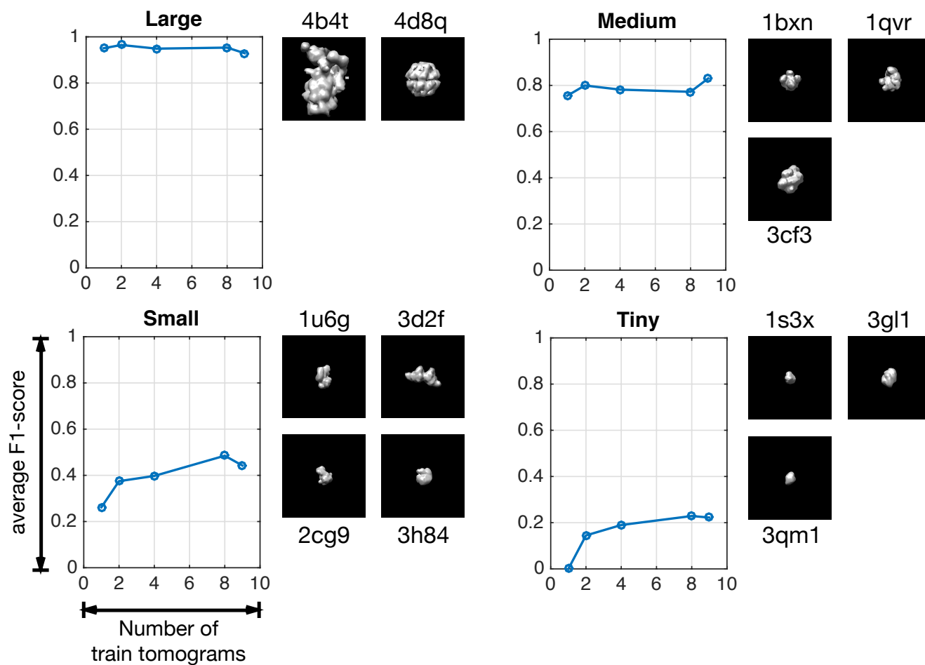
Figure 10: Evolution of F_1 -scores with respect to sizes of the training sets (number of tomograms) on the synthetic SHREC'19 dataset (12 classes). This figure gives an estimation of the amount of annotated data needed to identify macromolecules. This amount depends on the size of the target macromolecule: the smaller the target, the more annotations are required. Each tomogram contains in average 208 macromolecules per class. The macromolecules have been categorized into 4 groups (large, medium, small and tiny).
