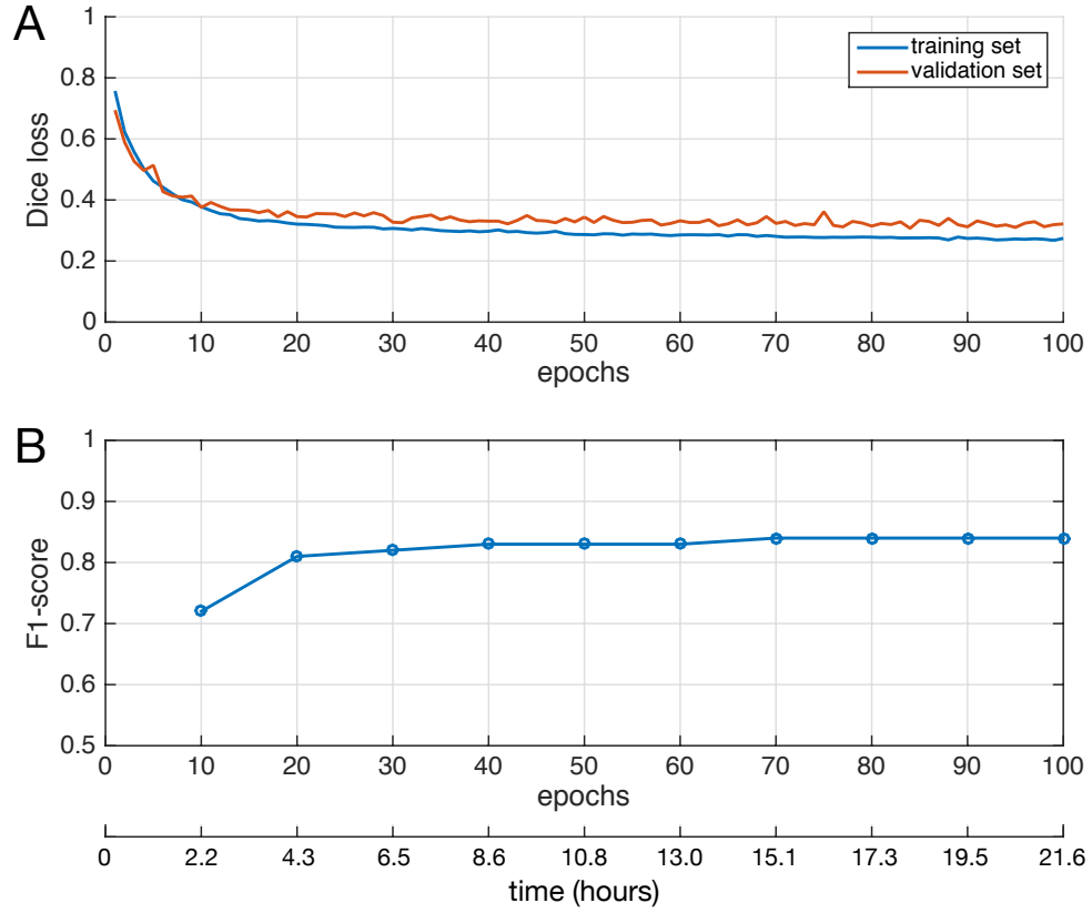
Figure 17: Evolution of loss and F_1 -score with respect to training iterations (Dataset #2). (A) The loss, which quantifies the segmentation quality, is computed for the training set, as well as for the validation set. Comparing both curves allows assessment of the generalization capabilities of our 3D CNN method. The curves for both sets should ideally overlap, otherwise it indicates overfitting (the network memorizes trained samples instead of learning discriminating features). One epoch equals to 100 training iterations. (B) The F_1 -score, which quantifies the localization performance, computed on the test set. The time axis has been obtained using a Tesla K80 GPU. The curve indicates that competitive particle picking results are obtained after 20 epochs, or 4.3 hours with the required GPU.
