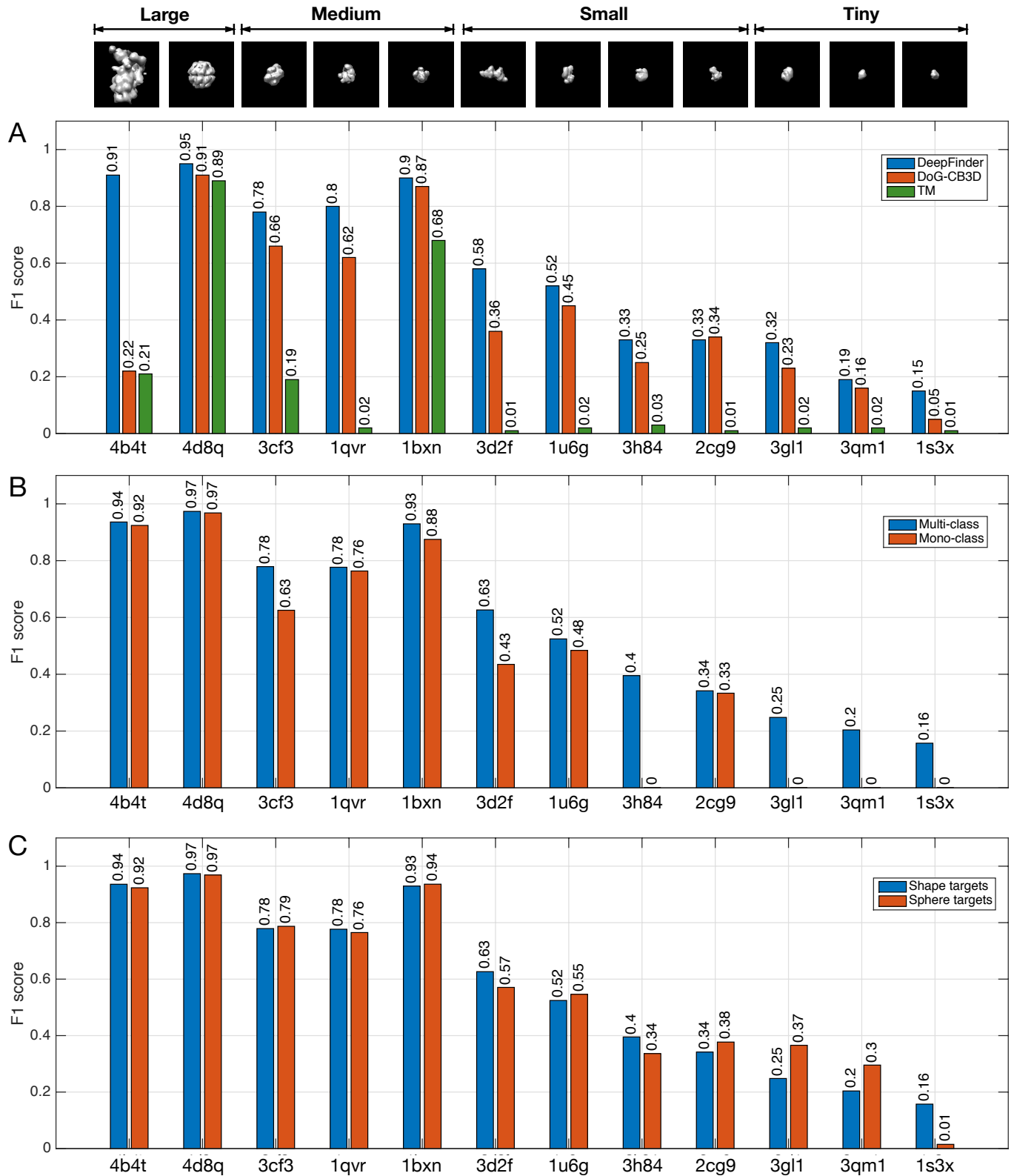
Figure 3: Analysis of algorithm performance on the synthetic dataset (SHREC'19 challenge). (A) Performance ( F_1 -score) of DeepFinder, DoG-CB3D and template matching algorithms and ability to discriminate between 12 classes/subclasses of macromolecules. The tiny macromolecules are 1s3x (human Hsp70 ATPase domain), 3qm1 (Lactobacillus Johnsoni Cinnsmoyl esterase LJ0536 S106A mutant in complex Ethylferulate Form II), and 3gl1 (Saccharomyces cerevisiae ATPase domain of Ssb1 chaperone). The highest possible value of an F_1 -score is 1.0 and the lowest possible value is 0. The scores of template matching were provided by the SHREC'19 challenge organizers (Utrecht University, Department of Information and Computing Sciences and Department of Chemistry). (B) Performance of DeepFinder implemented as a multi-class network architecture and as an architecture made of 12 binary networks. These two architectures differ only by the number of output neurons. (C) Influence of the training target generation method ("shapes" versus "spheres"). In the case of "shapes", the exact shapes of the macromolecules have been used to annotate the tomograms. In the case of spheres", the shape and the orientation of macromolecules are not needed to generate the training targets.
