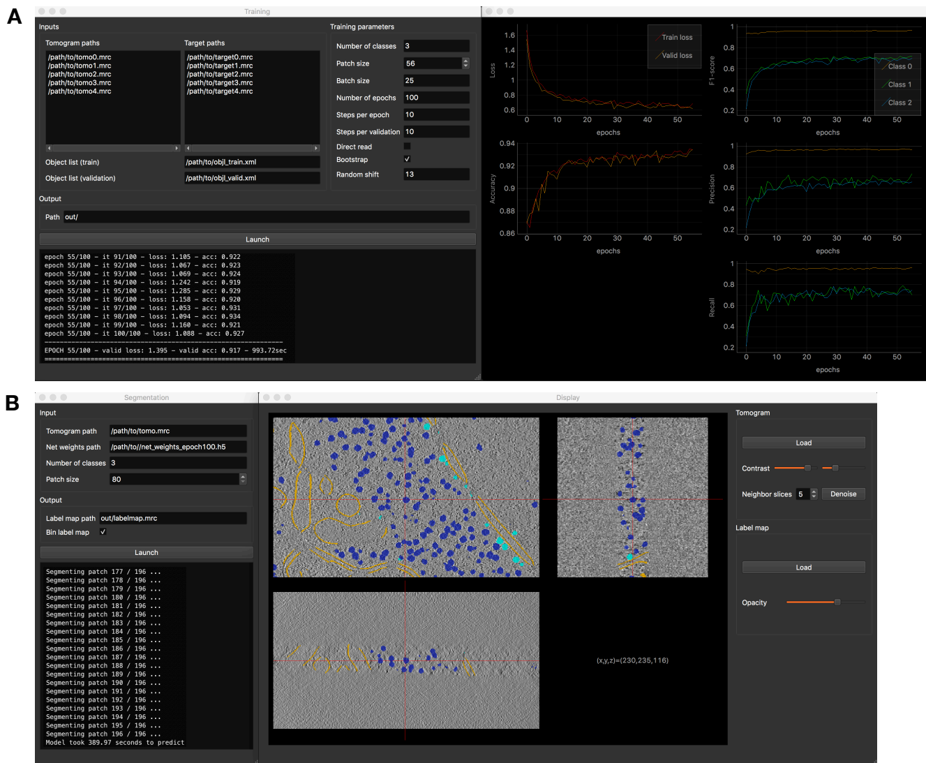
Figure 6: DeepFinder graphical user interface. (A) Training interface composed of a first window for parametrizing the procedure and a second window for displaying the training metrics in real-time. (B) Segmentation interface which also opens a data visualization tool. This tool allows one to explore the tomogram with superimposed segmentations. In addition, DeepFinder also incorporates interfaces for tomogram annotation, target generation and clustering (see the documentation at https://gitlab.inria.fr/serpico/deep-finder for more information).
