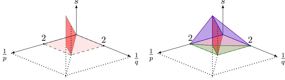
FIGURE 5. Parameter domain for F -spaces in Steps 1 and 2 (left figure), and after the interpolation argument in Step 3 (right figure) of the proof of Proposition 4.5.
